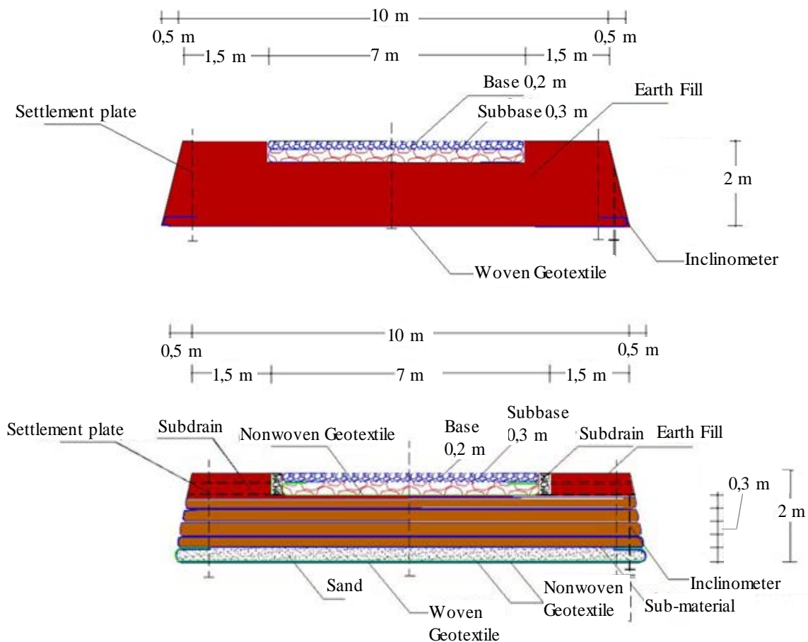
Fig.3 Embankment with Sub-material
