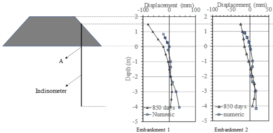
Fig.6 Horizontal Displacement Results
