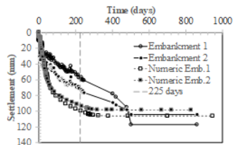
Fig.5 Time-Average Settlement Curves Obtained by Numeric and Settlement Plate Measurement
