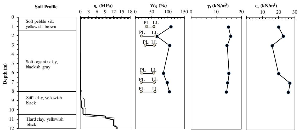
Fig.1 Soil layer profile, CPT result, and other soil nature
