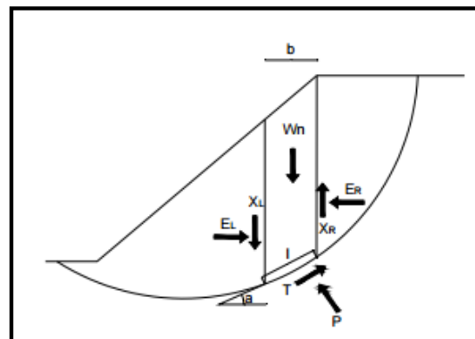
Figure 4. Force working on the sliced area.
