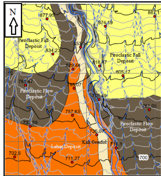
Figure.5 Geological map
