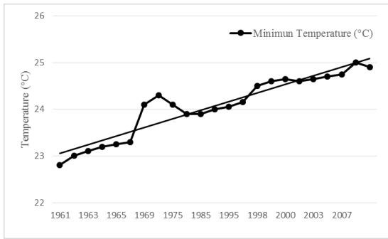
Fig. 2 Average minimum temperatures in Bangkok, 1961-2007.
