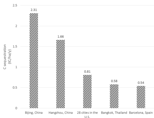
Fig. 4 Comparison of carbon sequestration in study area and previous research
