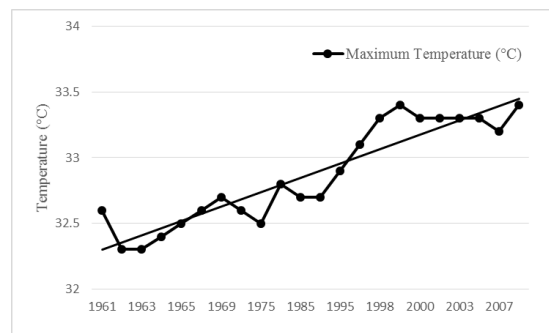
Fig. 1 Average maximum temperature in Bangkok, 1961-2007.
