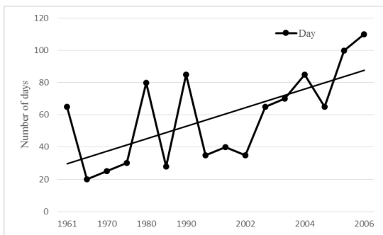
Fig. 3 Number of days exceeding 35°C in Bangkok, 1961-2007.
