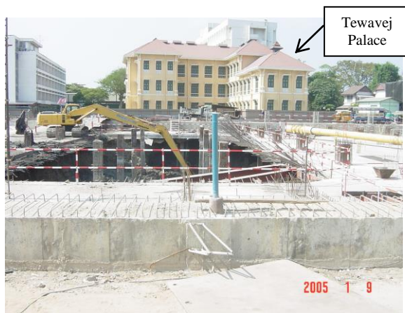
Fig. 9 Photograph during excavation closed to Tewavej Palace
