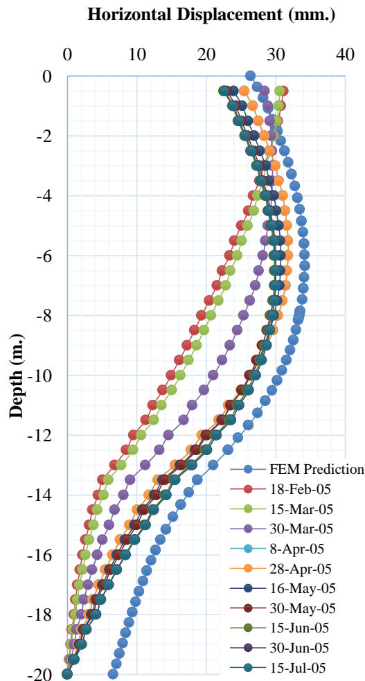
Fig. 8 The inclinometer I-3 monitoring results with the predicted maximum movement by FEM analysis.
