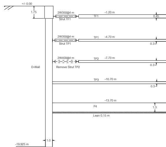
Fig. 3 Typical section of underground basement
