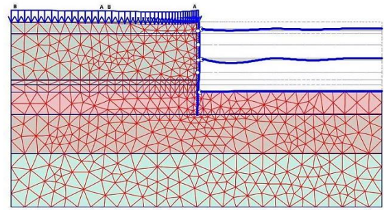
Fig. 7 Deformed mesh of FEM analysis at the final stage excavation at -15.6m.
