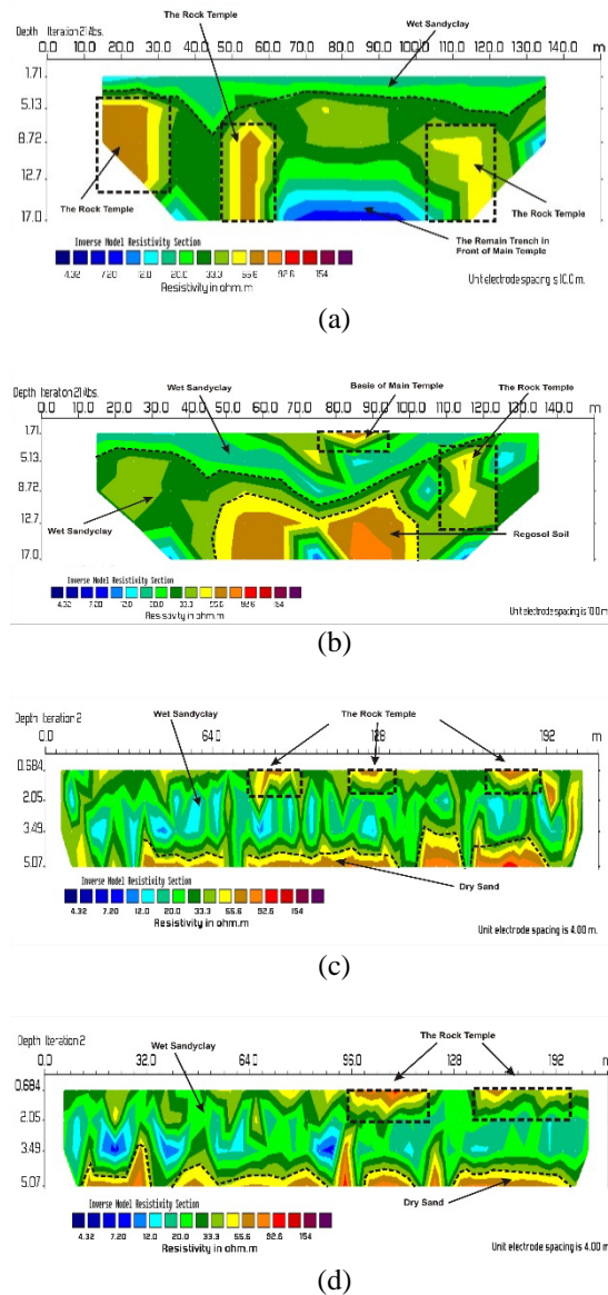
Fig. 6 Two Dimension (2D) Resistivity Cross Section (a) Line 7, (b) Line 8, (c) Line 9, and (d) Line 10
