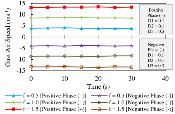
Fig.9 Gust air speed versus time with regards to an array of oscillation frequencies
