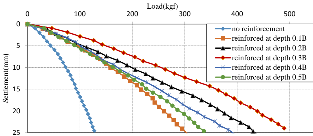
Fig.7 Load versus settlement curve for sand bed reinforced with geotextile of size 3Bx3B with prestressed
