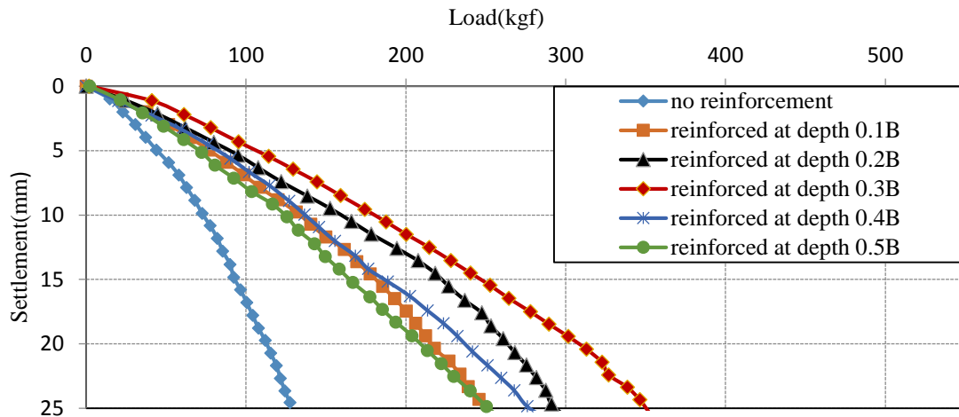
Fig.6 Load versus settlement curve for sand bed reinforced with geotextile of size 3Bx3B without prestressed
