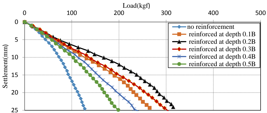
Fig.4 Load versus settlement curve for sand bed reinforced with geotextile of size 2Bx2B without prestressed
