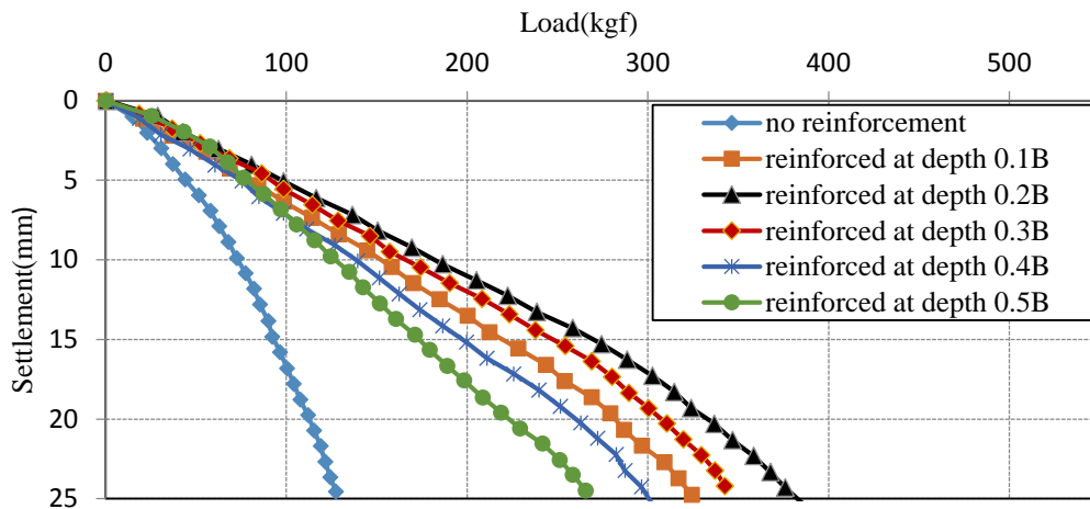
Fig.5 Load versus settlement curve for sand bed reinforced with geotextile of size 2Bx2B with prestressed
