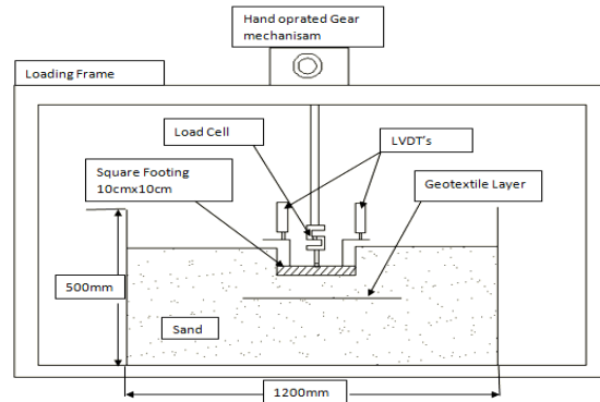
Fig.2 The schematic view of test apparatus
