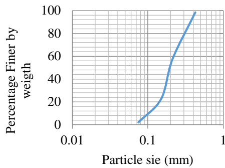
Fig.1 Grain size distribution curve for the sand
