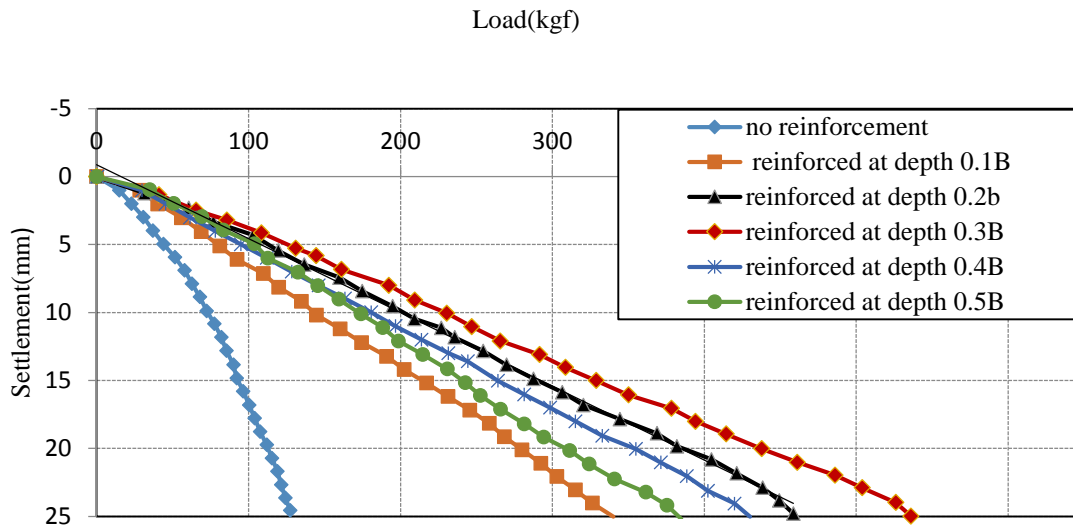
Fig.9 Load versus settlement curve for sand bed reinforced with geotextile of size 4Bx4B with prestressed
