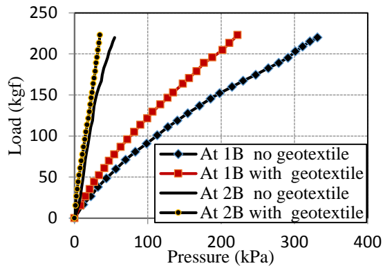
Fig.10 Load versus pressure cell reading
