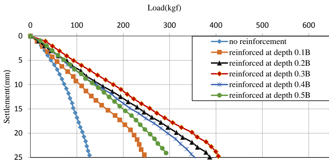
Fig.7 Load versus settlement curve for sand bed reinforced with geotextile of size 3Bx3B with prestressed
