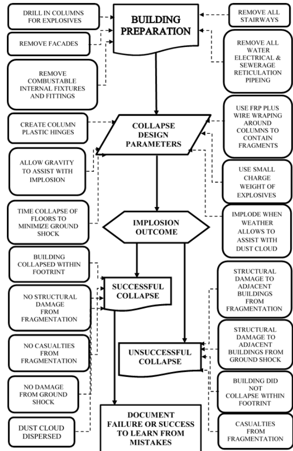
Fig. 3 Controlled demolition design process flowchart
