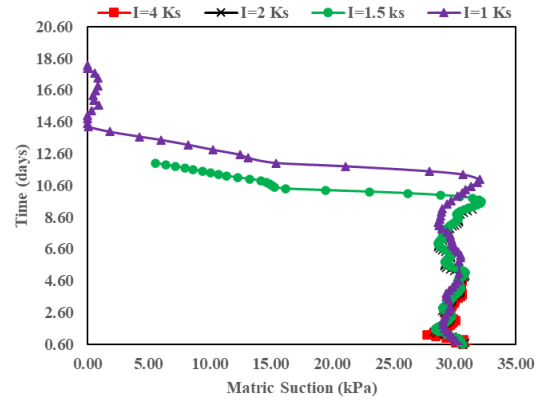
Fig.8c Matric suction response at depth 3
