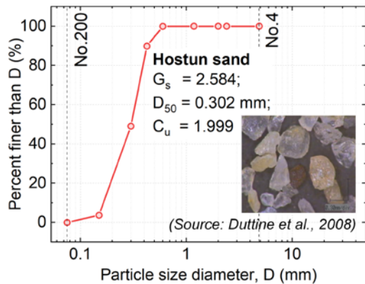
Fig. 1 Gradation curve and particle shape of Hostun sand used in present study (modified from Dutti et al. [28])
