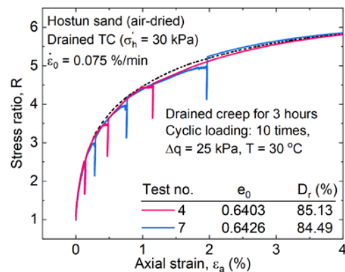
Fig. 10 R - \varepsilon_a relationships with loading type b) SL-CL with T = 30^\circ\text{C}
