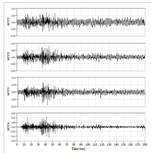
Fig.8. Results of single pile with Nelton geogrid (200×200 mm)
