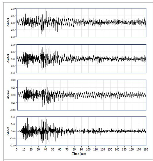
Fig.12. Results of single pile with SQ12 geogrid (700×700 mm)
