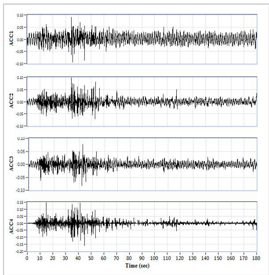
Fig.9. Results of single pile with SQ12 geogrid (200×200 mm)
