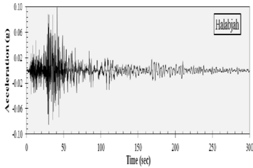
Fig.6. Acceleration with time for Halabjah earthquake
