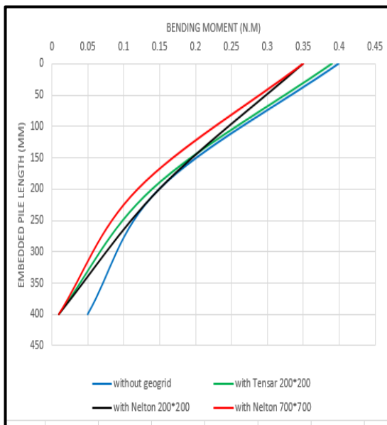
Fig.7. Bending moment vs embedded pile length
