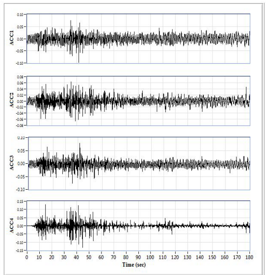
Fig.10. Results of single pile with Tensar geogrid (700×700 mm)
