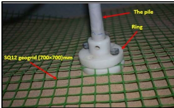
Fig 2c-d. Rings, mesh geogrid and the connections
