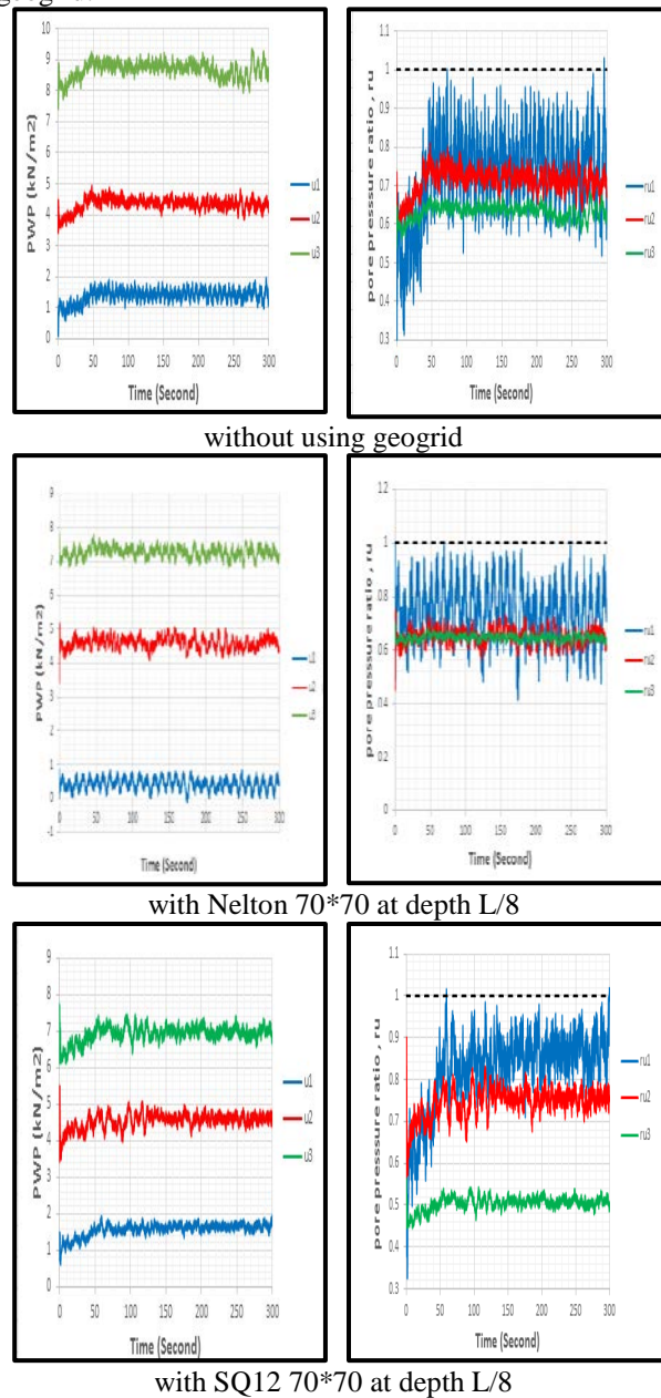
Fig.13. Excess pore water pressure with time in loose sand under Halabjah earthquake
