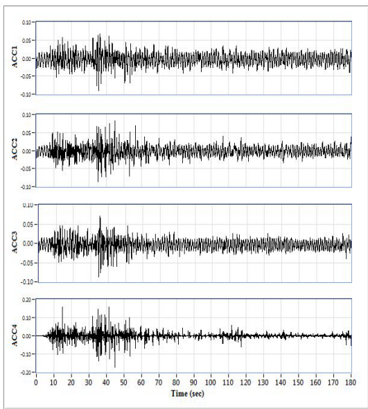
Fig.11. Results of single pile with Nelton geogrid (700×700 mm)
