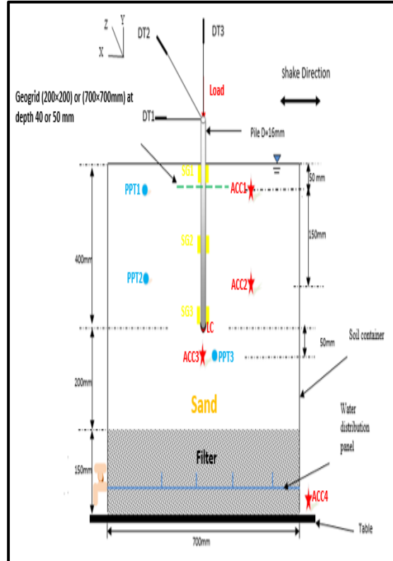
Fig.5. Sketch of laboratory test model
