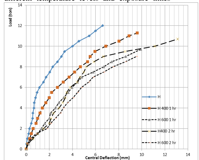
Fig. 9 Load-deflection curve for SCC beams under different temperature levels and exposure times
