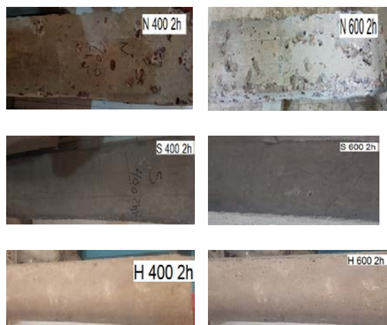
Fig. 5 Cracking phases for beams under different temperatures for 2 h exposure time
