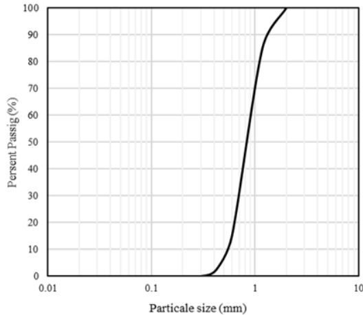
Fig. 7 Particle size distribution of the sand
