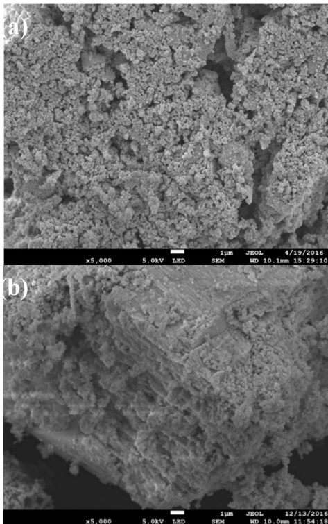
Fig. 6 Magnification of bauxite sample under 5000x magnification for (a) raw and (b) processed bauxite sample
