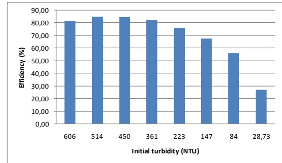
Fig. 7 Turbidity removal efficiency after using omhoff cone (represent sedimentation process)
