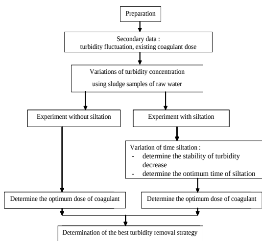
Fig. 1 Flowchart of research
