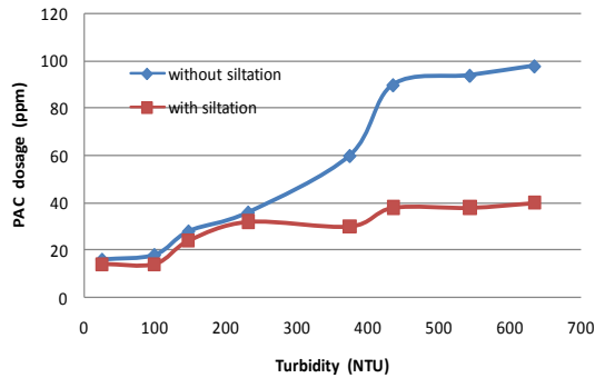
Fig.4 Coagulant dosage with and without siltation process
