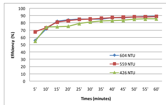
Fig. 6 Efficiency of turbidity reduction without siltation
