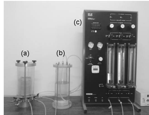
Fig. 1 Infiltration equipment. (a) Infiltration cell. (b) Transfer tank. (c) Pressure-volume panel
