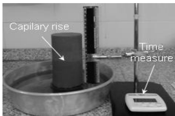
Fig.3 Capillary rise test
