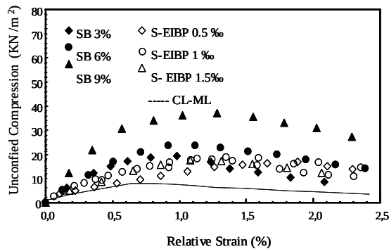
Fig.5 Unconfined compression test on soil /bentonite and soil / BPIS samples
