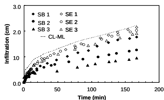
Fig. 4 Infiltration test on soil /bentonite and soil / BPIS samples
