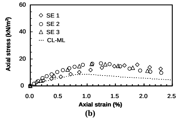
Fig. 6 Stress-strain curves unconfined compression test. (a) Soil/Bentonite. (b) Soil/BPIS
