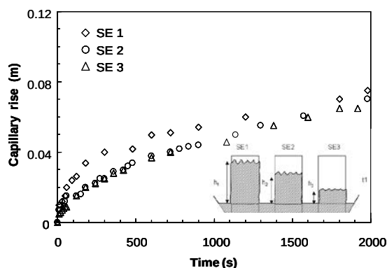
Fig. 8 Capillary rise Soil/BPIS
