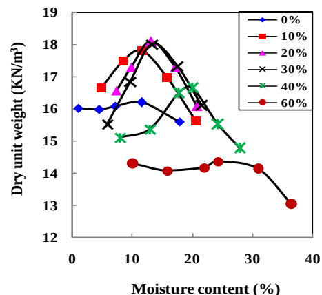
Fig.4 Compaction curves of sand-Al-Qatif clay mixtures with different clay contents
