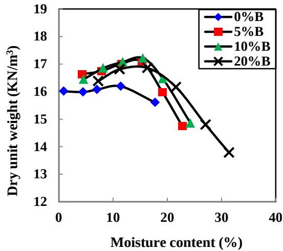
Fig.5 Compaction curves of sand-bentonite mixtures with different bentonite contents
