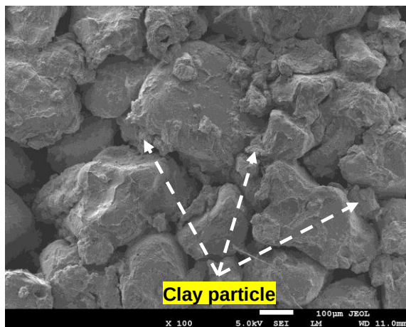
Fig.8 SEM of sand-bentonite mixtures mixture with 20% clay content
