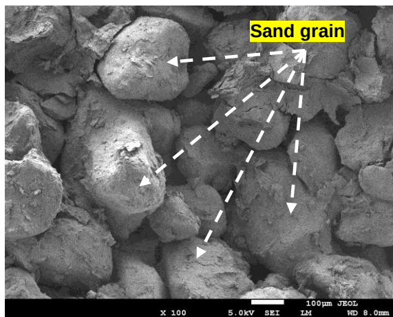
Fig.7 SEM of sand-Al-Qatif clay mixtures mixture with 20% clay content
