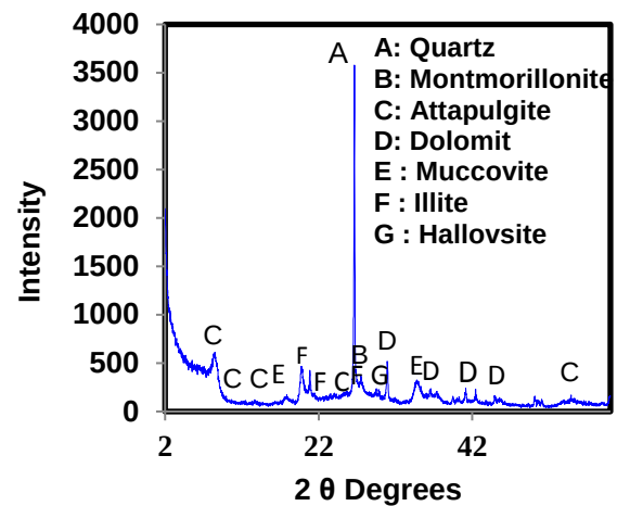
Fig.2 X-Ray diffraction of Al-Qatif clay
