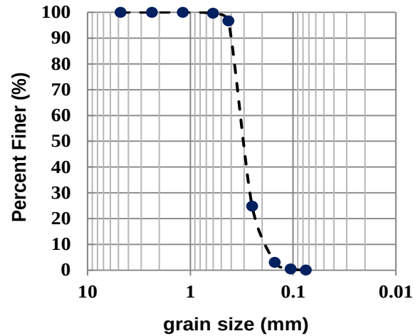
Fig.1 Grain size distribution of sand
