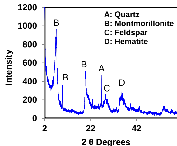
Fig.3 X-Ray diffraction of bentonite
