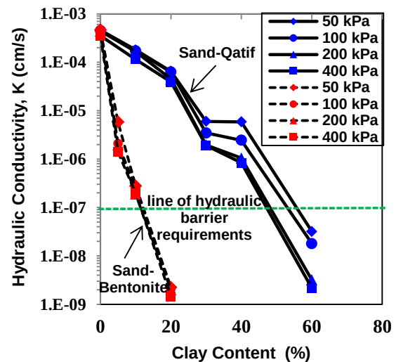
Fig.6 Variation of hydraulic conductivity of sand-Al-Qatif clay mixtures and sand-bentonite mixtures with clay content
