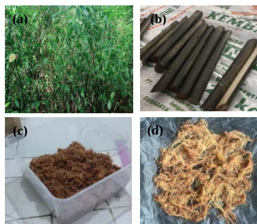
Fig. 1 Mechanism Process of Bemban Fiber: (a) Bemban plant; (b) Bemban stem cut from Bemban plant; (c) Bemban fiber before alkalization; (d) Bemban after alkalization
