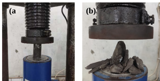
Fig. 7 Compressive strength test of geopolymer specimens: (a) Before test and (b) After test
